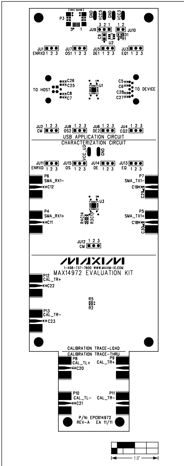
Figure 2. MAX14972 EV Kit Component Placement Guide—Component Side
