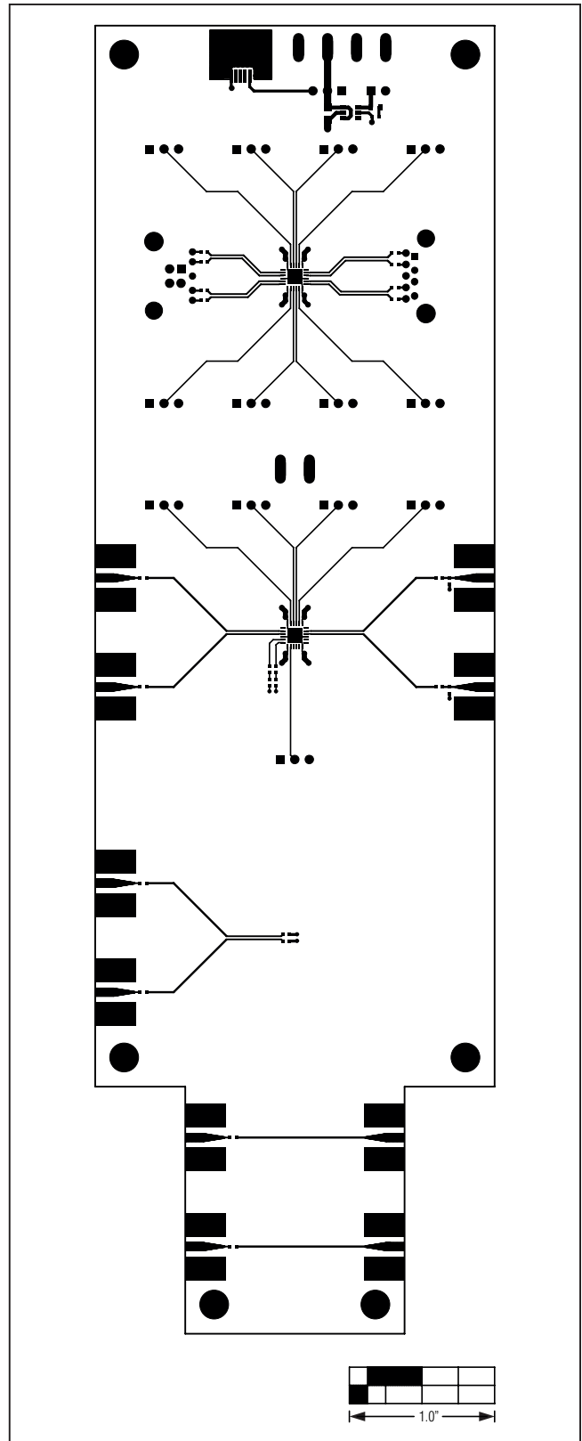
Figure 3. MAX14972 EV Kit PCB Layout—Component Side
