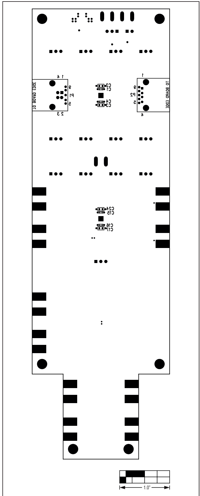
Figure 7. MAX14972 EV Kit Component Placement Guide—Solder Side
