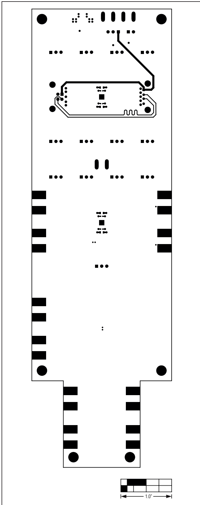
Figure 6. MAX14972 EV Kit PCB Layout—Solder Side
