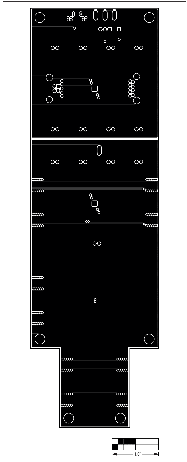
Figure 5. MAX14972 EV Kit PCB Layout—Inner Layer 3
