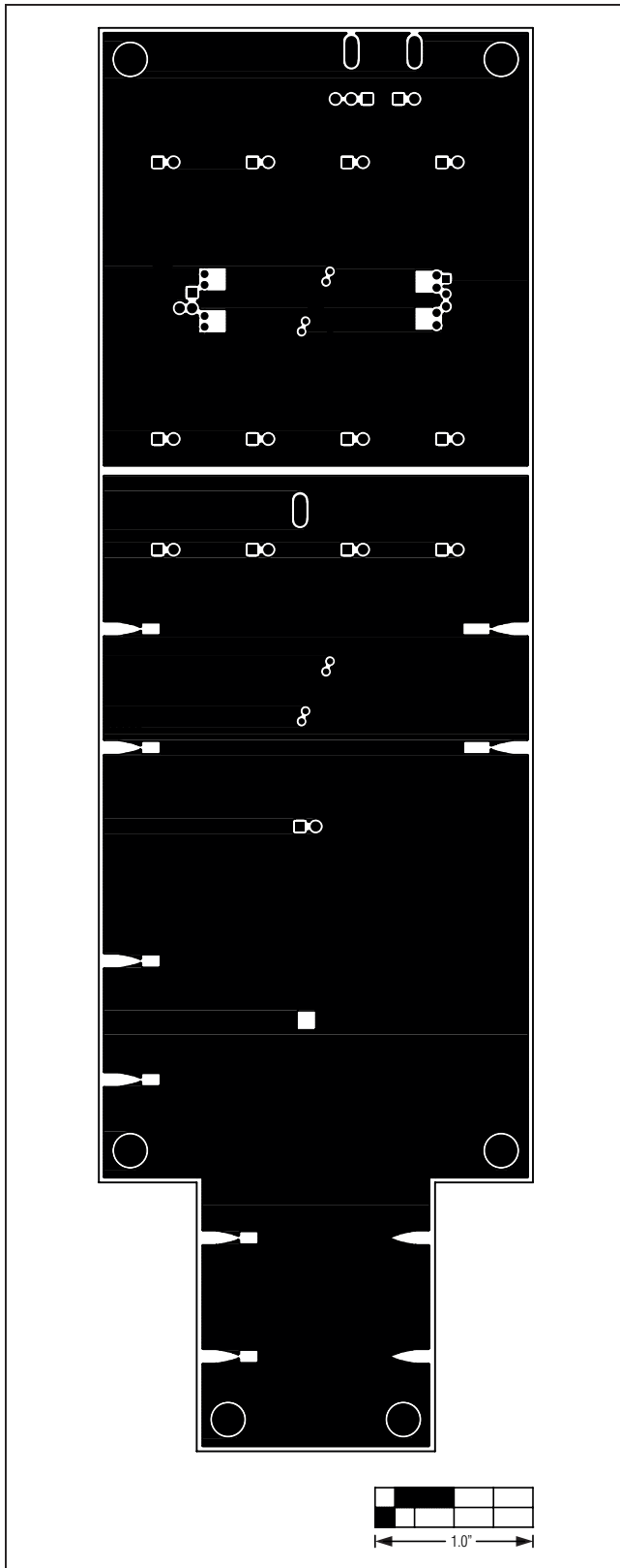
Figure 4. MAX14972 EV Kit PCB Layout—Inner Layer 2
