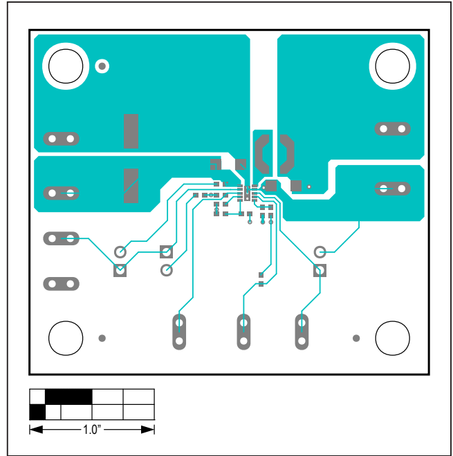
MAX17552A 5V EV Kit (TDFN)—Top Layer
