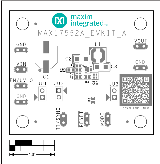
MAX17552A 5V EV Kit (TDFN)—Top Silkscreen
