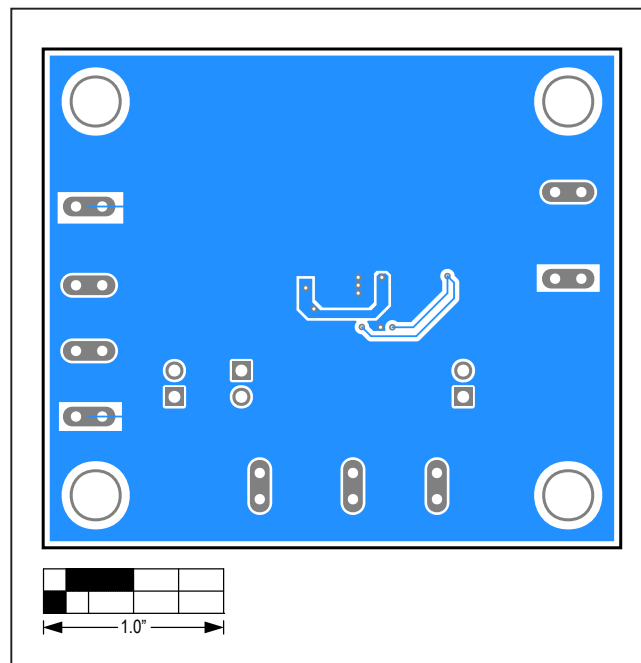
MAX17552A 5V EV Kit (TDFN)—Bottom Layer
