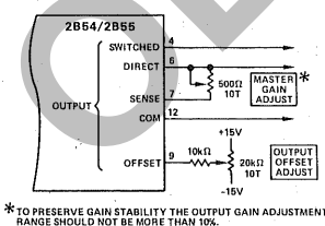
Figure 4. Output Offset and Master Gain Adjustments
