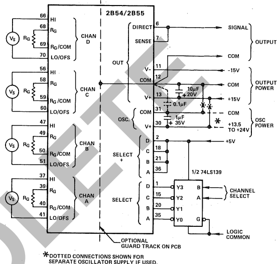
Figure 2. Basic 2B54/2B55 Application
