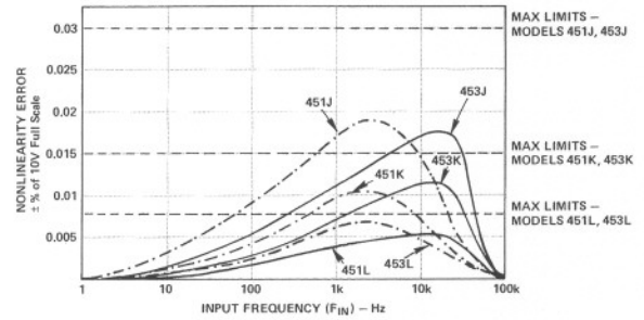
Figure 11. Nonlinearity Error Versus Input Frequency
