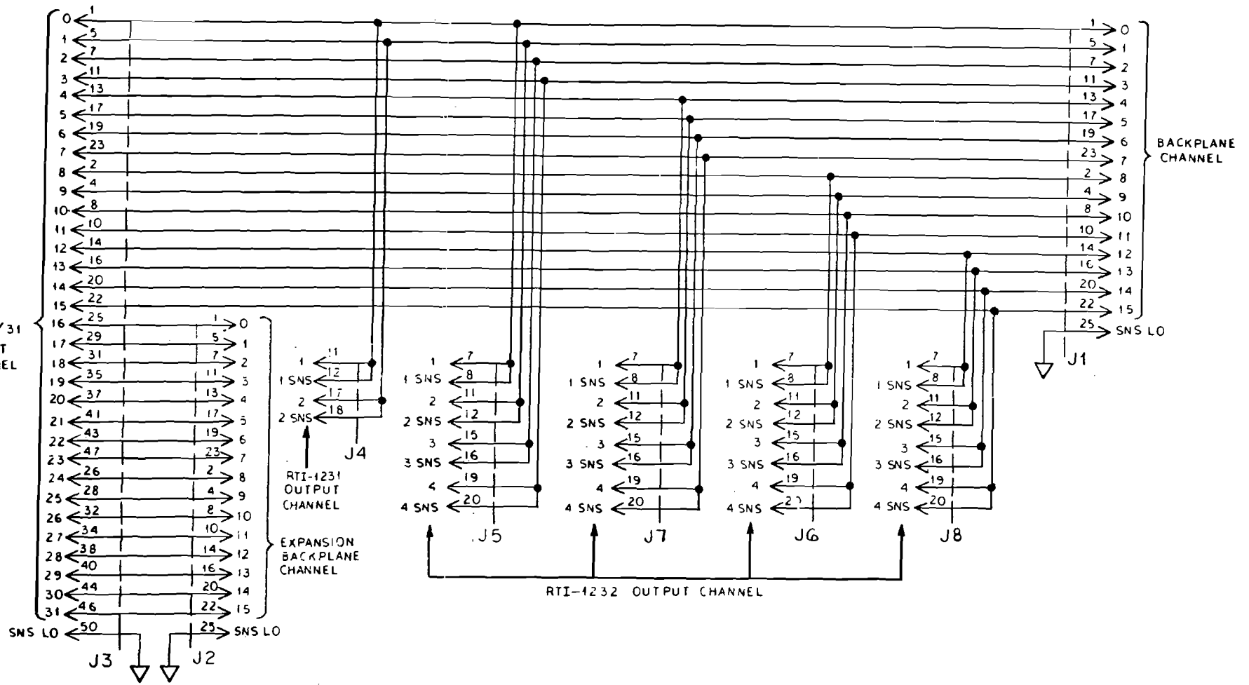
Figure 5.5 AC1321 Schematic
