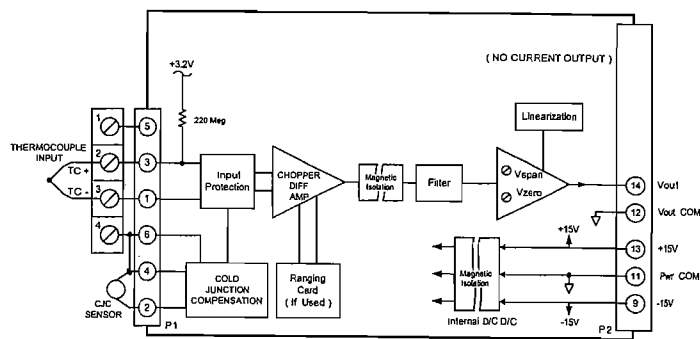
Figure 2.1.14.1 3B47 Functional Block Diagram
