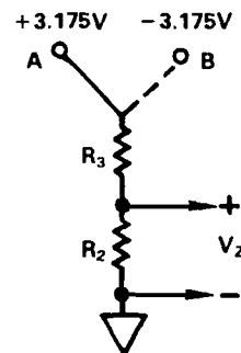
Figure 2.1.11.3 3B40 and 3B41 Zero Suppression Resistors
