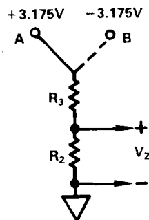
Figure 2.1.8.3 3B30 and 3B31 Zero Suppression Resistors
