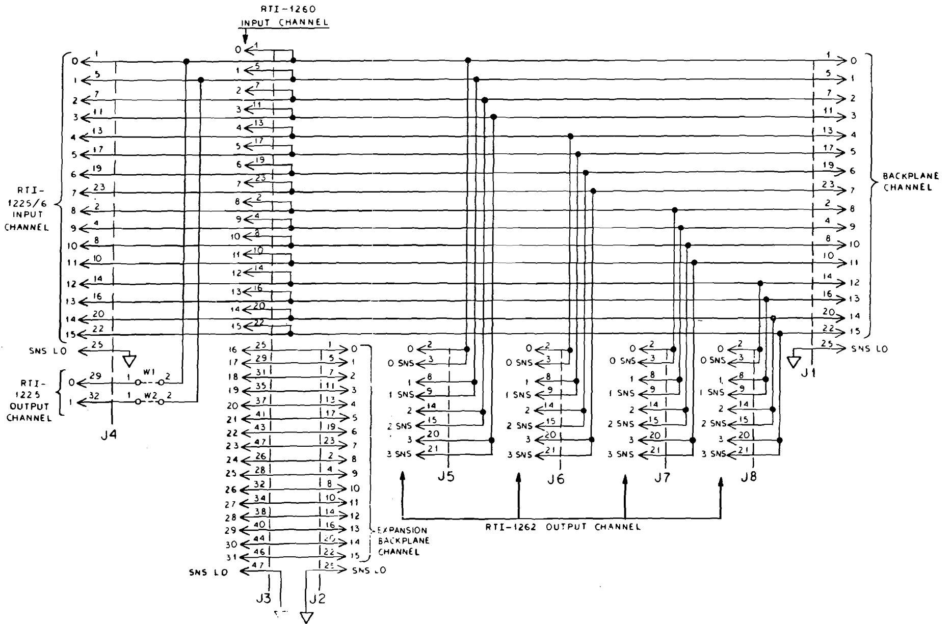
Figure 5.4 AC1320 Schematic
