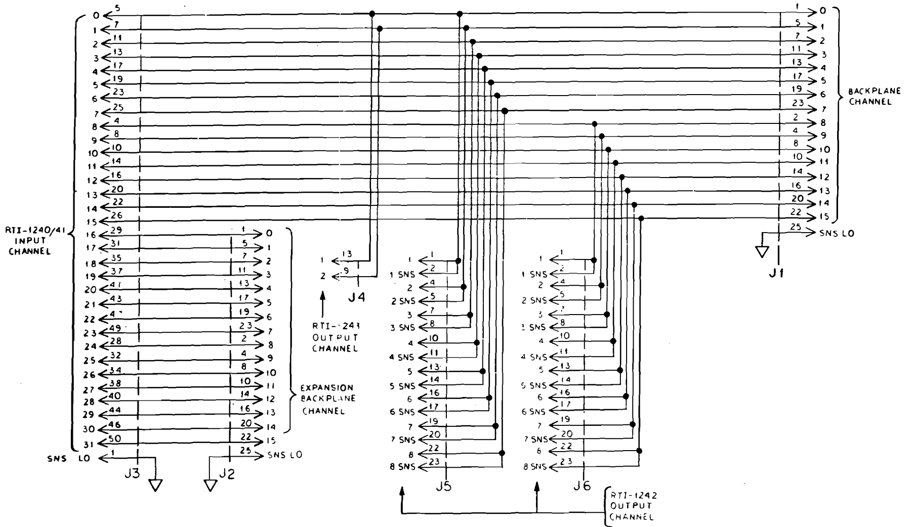
Figure 5.6 AC1322 Schematic
