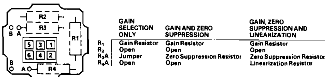
Figure 2.1.9.3 3B34 Custom Ranging
