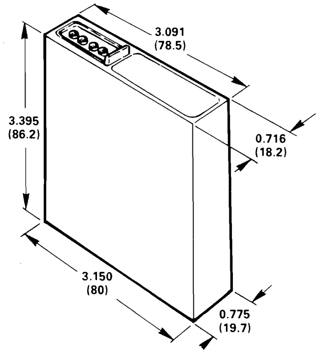
Figure 2.2.3 Output Module Dimensions Dimensions shown in inches and (mm).
