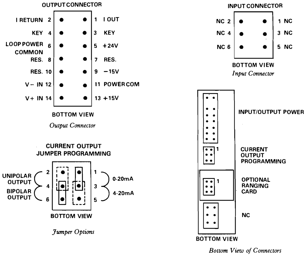
Figure 2.2.2 Output Module Connectors
