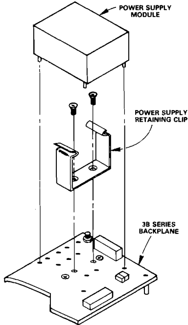
Figure 3.3.1 Power Supply Installation
