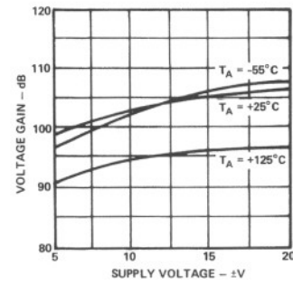
Voltage Gain
