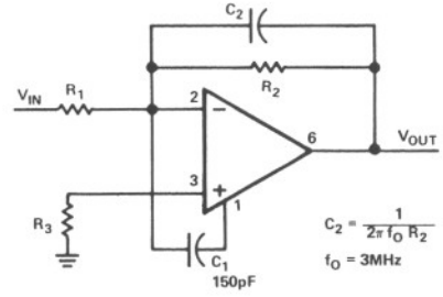
Figure 3. Feedforward Compensation
