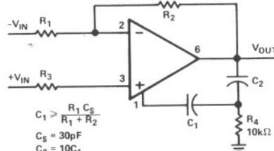
Figure 2. Two Pole Compensation
