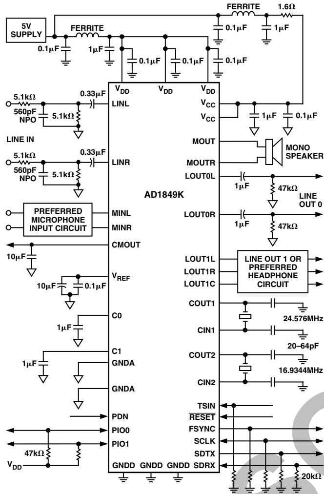
Figure 21. Typical Connection Diagram
