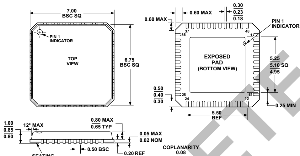
Figure 3. 48-Lead, Pb-Free, Frame Chip Scale Package [LFCSP_VQ] 7 mm x 7 mm Body, Very Thin Quad (CP-48-1)
