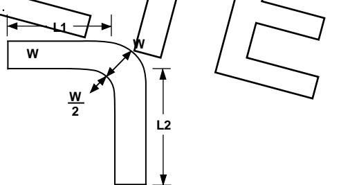
Figure 7. PCB Track Shunt Resistor with 90° Bend
