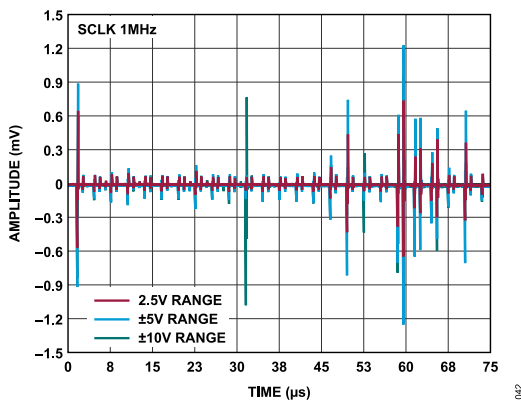
Figure 51. Digital Feedthrough
