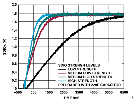
Figure 88. Driving Strength Options
