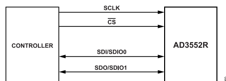
Figure 81. Dual SPI Connection
