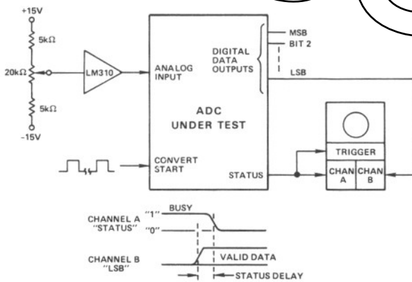
Figure 4. ADC Status Valid Test
