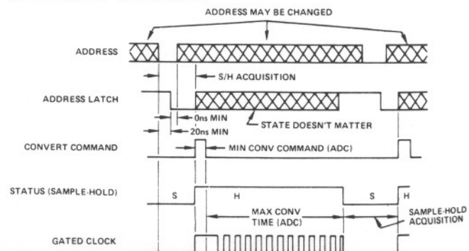
Figure 3. DAS Timing Diagram
