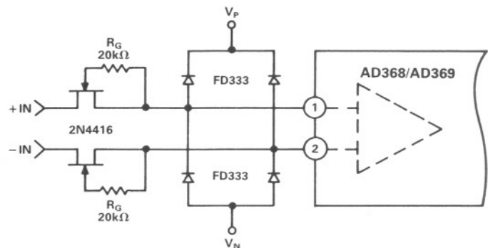
Figure 11. Low Noise Input Protection Circuit for AD368/AD369
