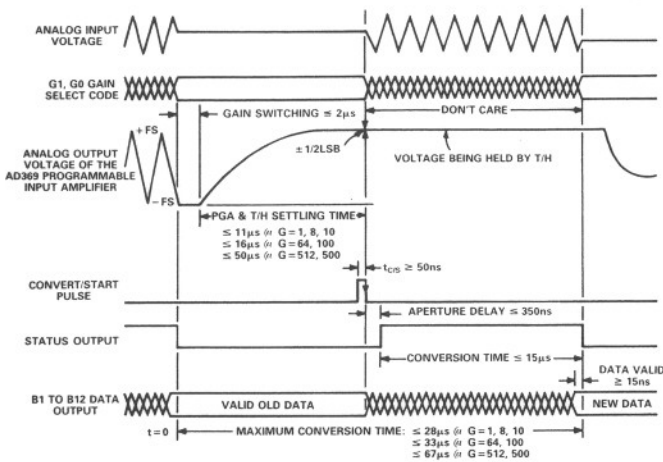
Figure 1a. AD368/AD369 Timing Diagram Without Pipelining
