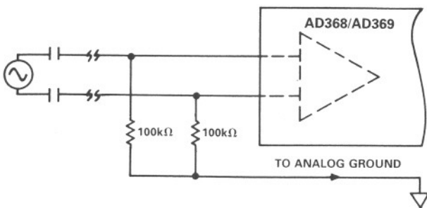
Figure 13b. Ground Returns for Bias Currents with ac Coupled Inputs
