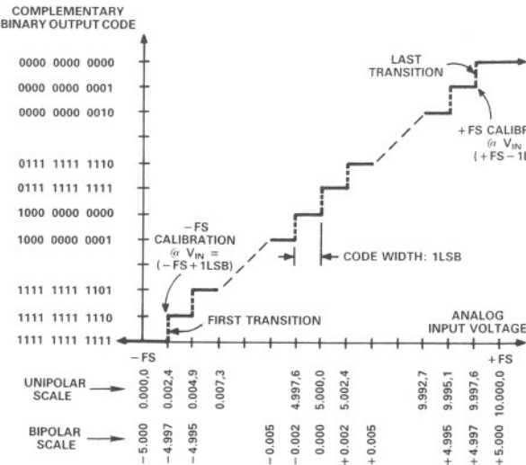
Figure 2. AD368/AD369 Transfer Function
