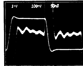
Figure 25c. Unity Gain Inverter Small Signal Response
