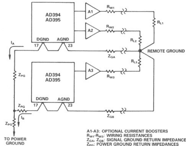
Figure 8. Grounding Errors in Multiple-AD394, AD395 Systems
