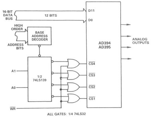
Figure 12. AD394, AD395 16-Bit Bus Interface
