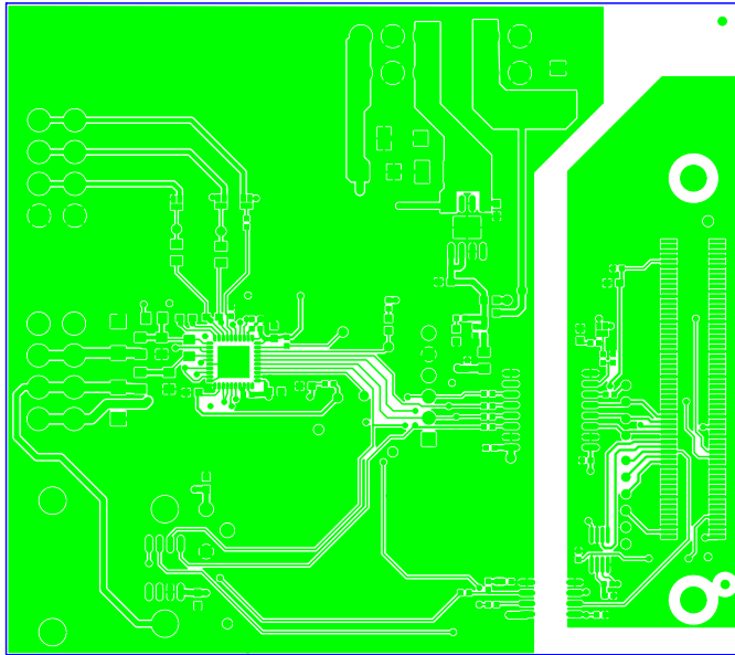
EVAL-AD4110-1SDZ (Rev. A) - Component Side View Layer 1 - Component Side Drill Template
