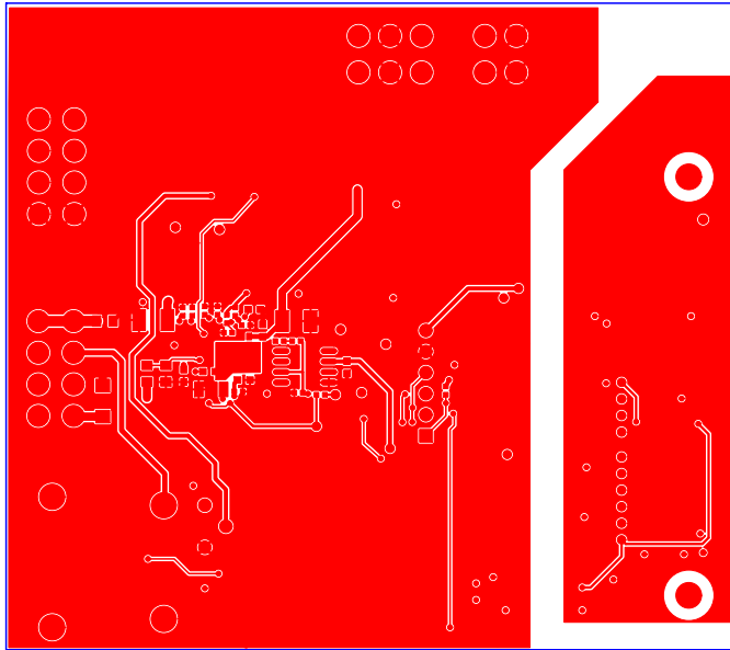
EVAL-AD4110-1SDZ (Rev. A) - Component Side View
