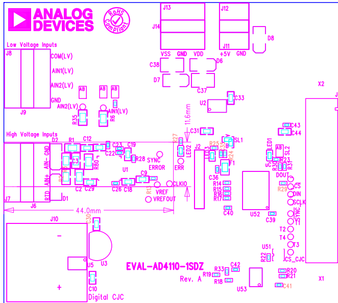
FID5 EVAL-AD4110-1SDZ (Rev. A) - Component Side View Layer 1 - Component Side Drill Template Silkscreen
