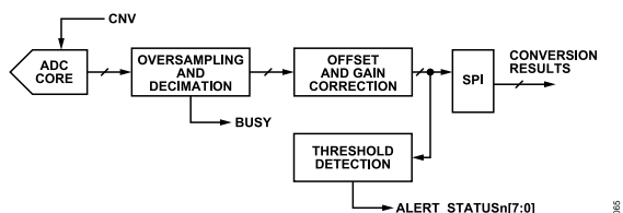
Figure 64. ADC Data Processing Path
