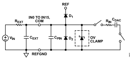
Figure 66. Equivalent Analog Input Circuit
