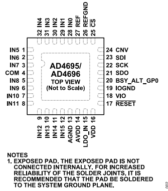
Figure 2. AD4695/AD4696 LFCSP Pin Configuration
