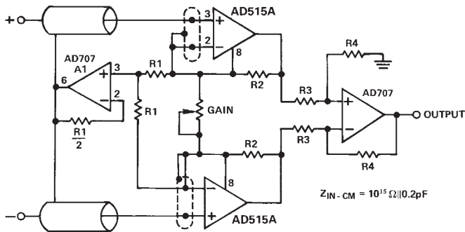
Figure 11. Very High Impedance Instrumentation Amplifier
