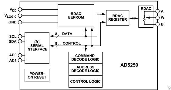
Figure 1. Block Diagram
