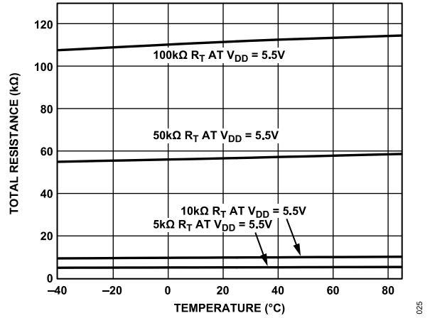
Figure 21. Total Resistance vs. Temperature
