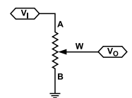
Figure 40. Potentiometer Mode Configuration
