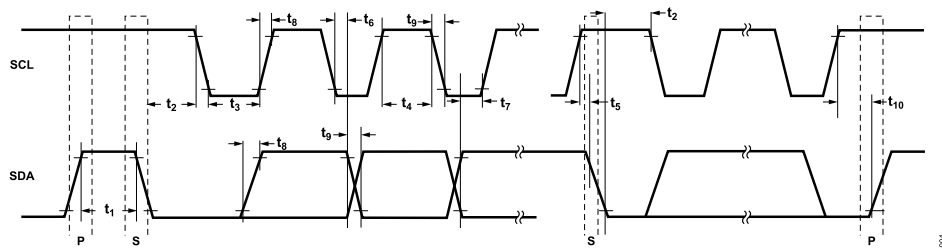
Figure 4. I 2 C Interface Timing Diagram
