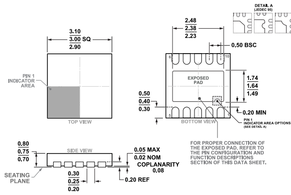
Figure 49. 10-Lead Lead Frame Chip Scale Package [LFCSP] 3 mm x 3 mm Body and 0.75 mm Package Height (CP-10-9) Dimensions shown in millimeters
