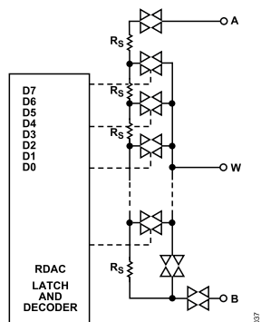
Figure 39. AD5259 Equivalent RDAC Circuit
