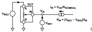
Figure 34. Test Circuit for Wiper Resistance
