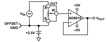
Figure 36. Test Circuit for Gain vs. Frequency
