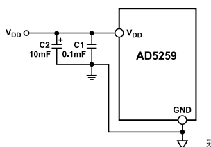
Figure 44. Power Supply Bypassing
