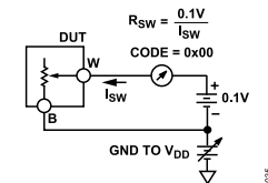
Figure 37. Test Circuit for Common-Mode Leakage Current
