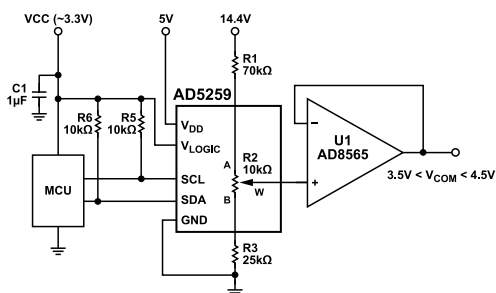
Figure 46. V_{\text{COM}} Adjustment Application
