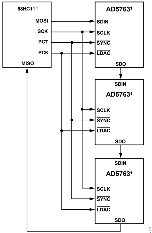
1 ADDITIONAL PINS OMITTED FOR CLARITY. Figure 26. Daisy-Chaining the AD5763
