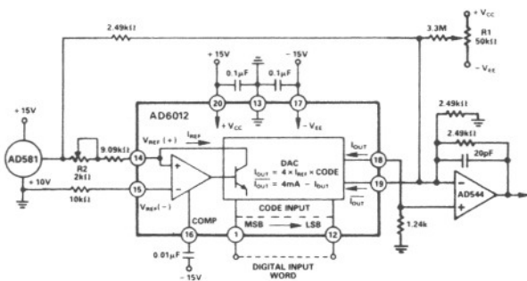
Figure 5. Negative Unipolar 0V to -10V
