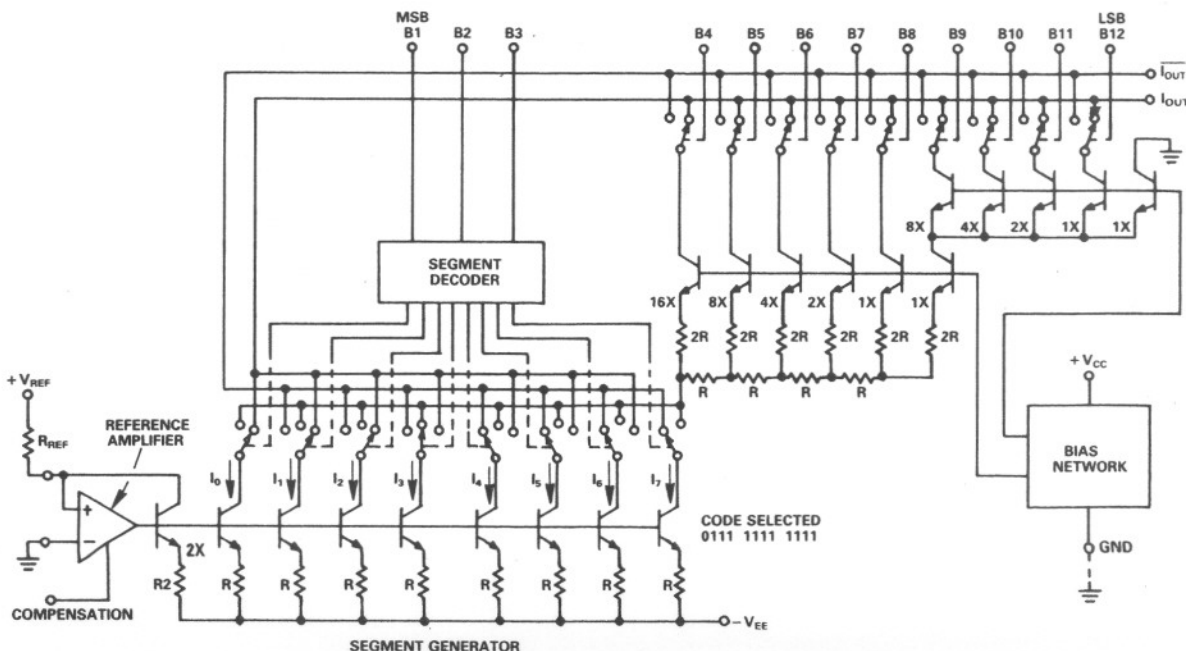
Figure 1. AD6012 Functional Block Diagram
