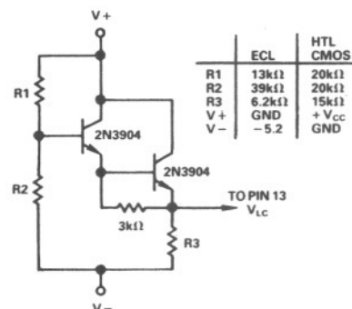
Figure 11. HTL, CMOS, or ECL Bias Circuit
