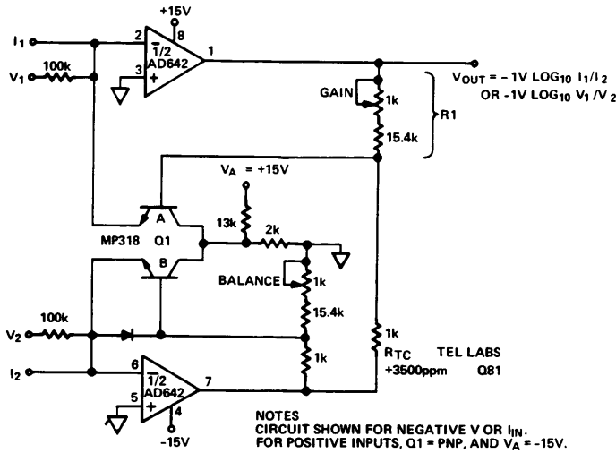
Figure 28. Log-Ratio Amplifier
