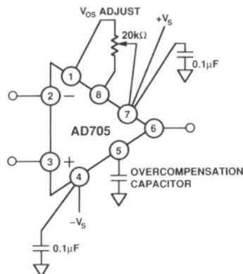
Figure 24. Offset Null and Overcompensation Connections
