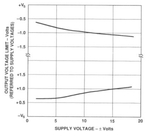
Figure 18. Output Voltage Limit vs. Supply Voltage
