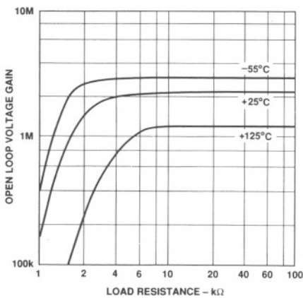
Figure 16. Open Loop Gain vs. Load Resistance over Temperature
