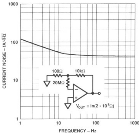
Figure 11. Input Noise Current Spectral Density
