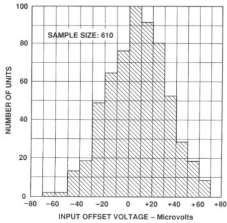
Figure 1. Typical Distribution of Input Offset Voltage
