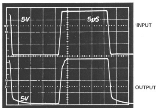
Figure 23b. Follower Feed-Forward Pulse Response
