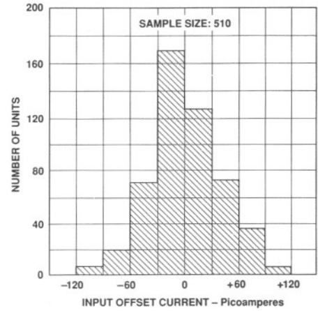
Figure 3. Typical Distribution of Input Offset Current
