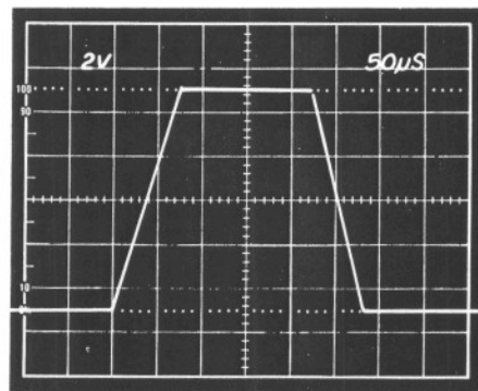
Figure 22b. Unity Gain Inverter Large Signal Pulse Response C_L = 50 pF
