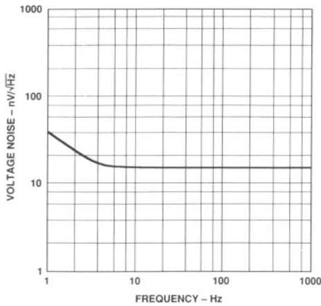
Figure 10. Input Noise Voltage Spectral Density
