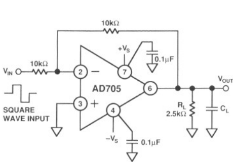
Figure 22a. Unity Gain Inverter
