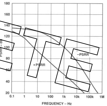
Figure 15. Power Supply Rejection vs. Frequency
