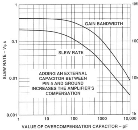
Figure 19. Slew Rate & Gain Bandwidth Product vs. Value of Overcompensation Capacitor
