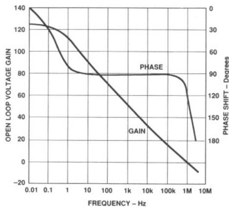
Figure 17. Open Loop Gain and Phase vs. Frequency
