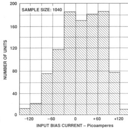
Figure 2. Typical Distribution of Input Bias Current
