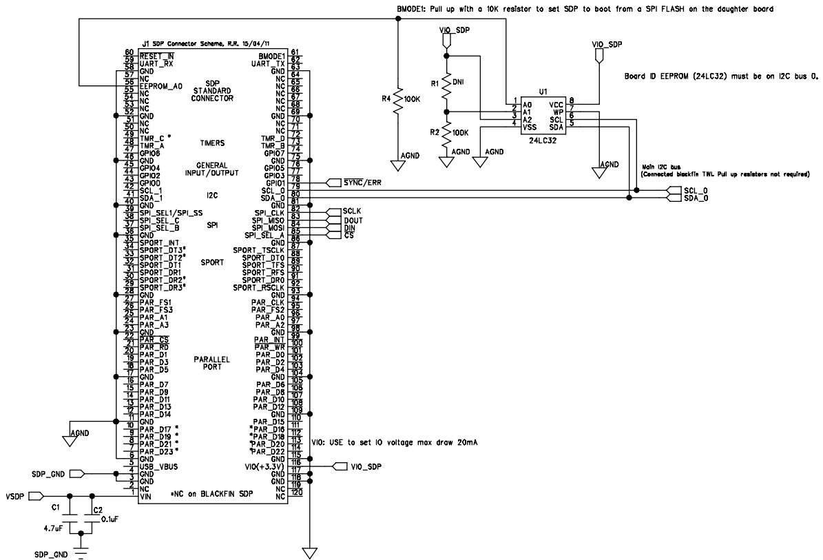
Figure 28. SDP-B Connector Schematic
