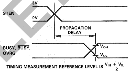
STEN to BUSY, \overline{BUSY} , or OVRG Propagation Delays
