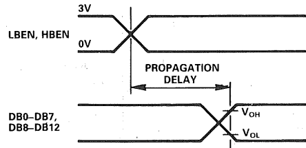
LBEN to DB0-DB7, HBEN to DB8-DB12 Propagation Delays
