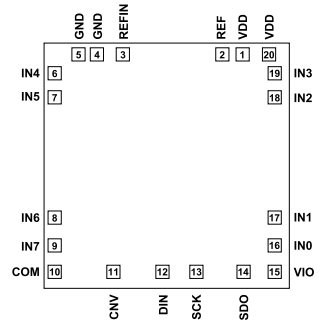
Figure 4. Pad Configuration
