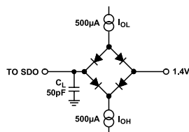
Figure 2. Load Circuit for Digital Interface Timing
