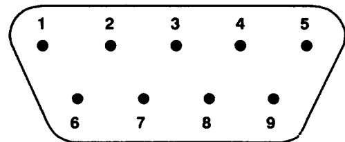
Figure 2. Pin Configuration for SKT1, D-Type Connector
