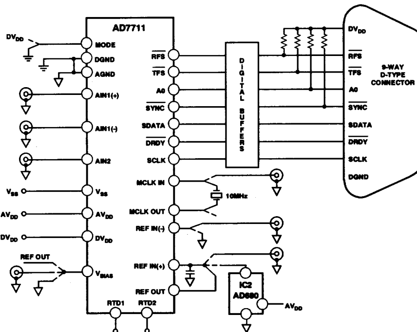
Figure 1. Evaluation Board Basic Schematic Diagram
