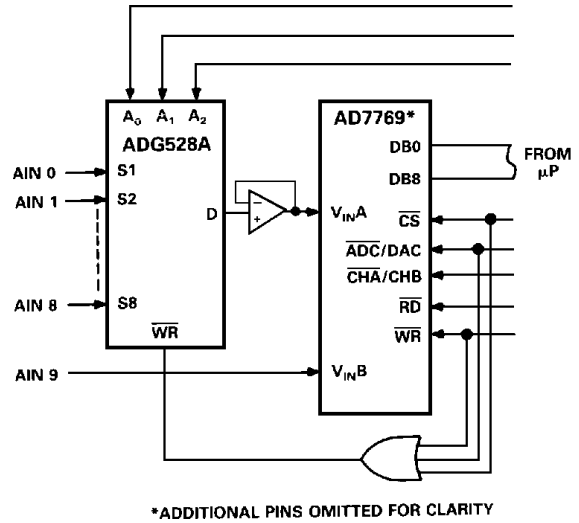
Figure 31. Multichannel Inputs
