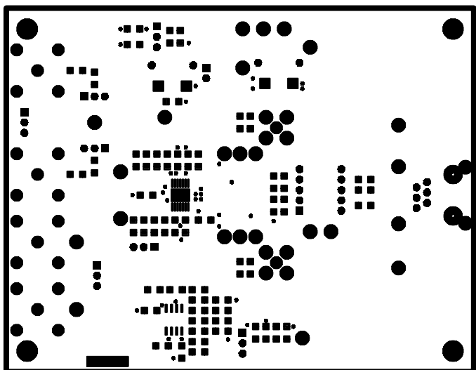
Figure 13. Solder Mask Top
