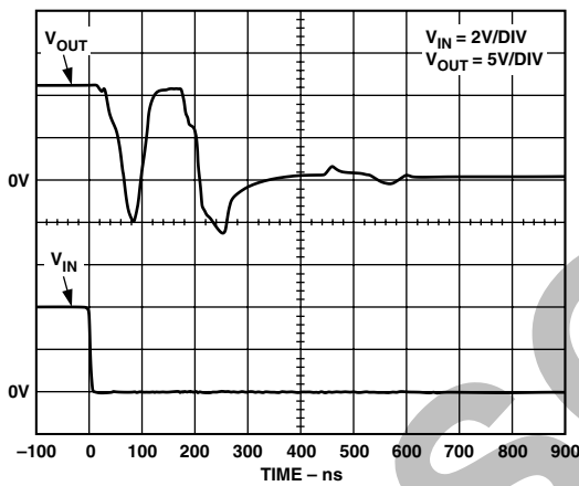
TPC 26. Overload Recovery; V_S = \pm 12\text{ V} , G = +5 , R_L = 100\ \Omega
