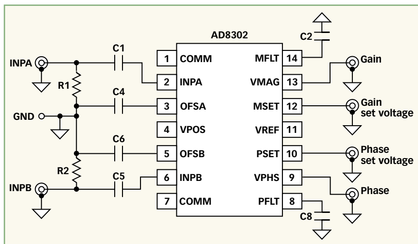
4. In the open-loop controller mode, the amplitude and phase outputs of the AD8302 are analogous to comparators.
