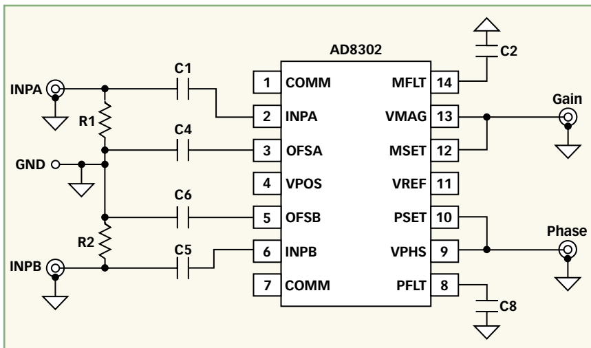
2. In the measurement mode, the AD8302's gain and phase outputs vary as a function of the gain and phase relationships between the input signals.
