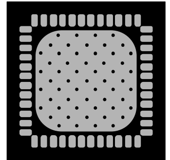
SOLDER MASK – TOP LAYER
