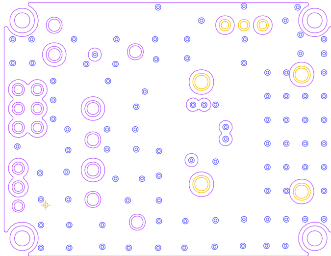
Figure 8. Evaluation Board Layout, Ground Plane (Layer 2)
