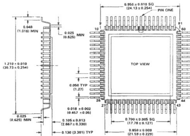
Leaded Ceramic Chip Carrier Suffix Z
