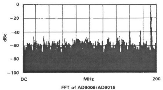
400MSPS: F_{IN} = 192\text{MHz} ; V_{IN} = 1.0\text{dB Below FS}
