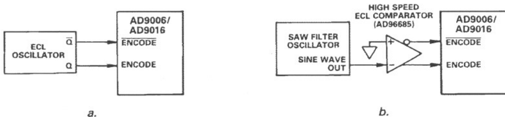
Figure 3. Clock Circuits
