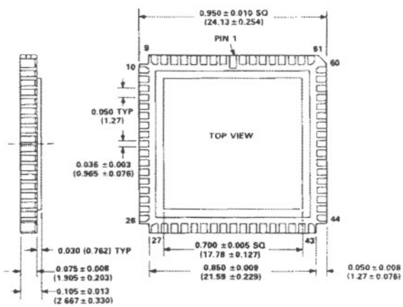
Leadless Chip Carrier (LCC) Suffix E
