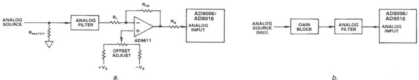
Figure 2. Analog Input Circuits
