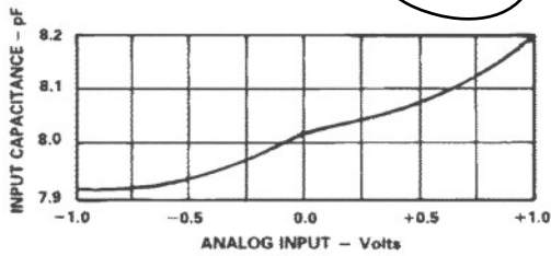
Input Capacitance vs. Input Voltage
