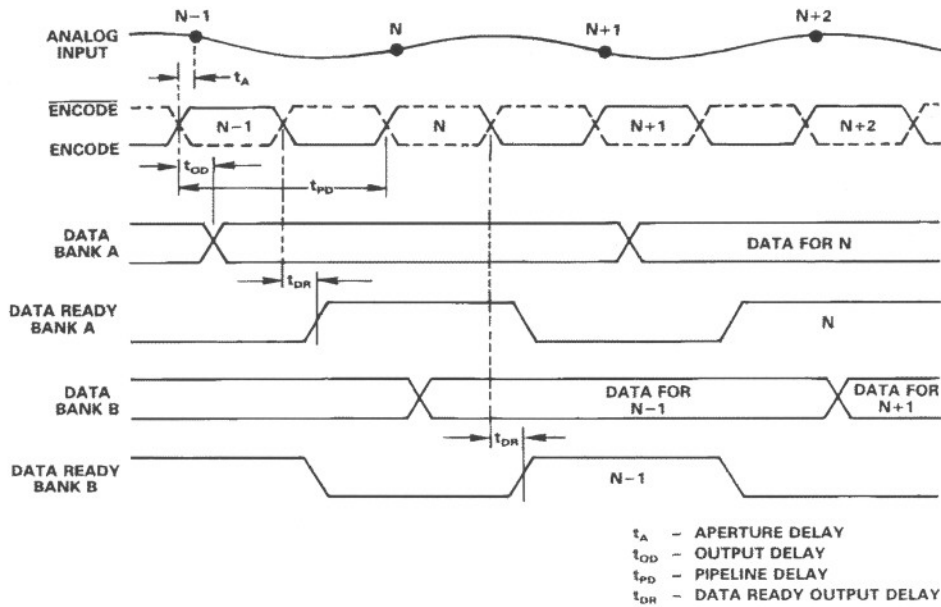
AD9016 Timing Diagram
