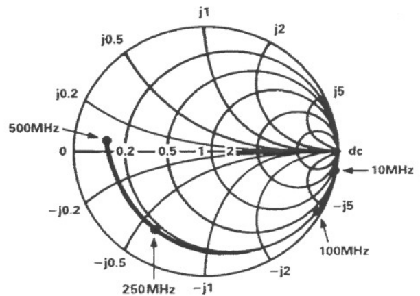
Normalized 50Ω Input Impedance vs. Input Frequency
