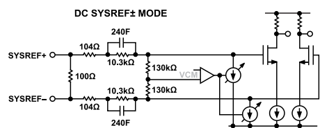
Figure 53. DC-Coupled SYSREF \pm Receiver Circuitry
