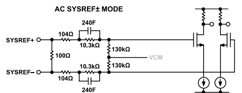
Figure 54. AC-Coupled SYSREF \pm Receiver Circuitry
