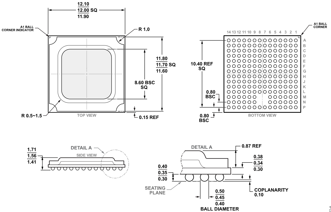
Figure 41. 192-Ball Ball Grid Array, Thermally Enhanced [BGA_ED] (BP-192-1)
