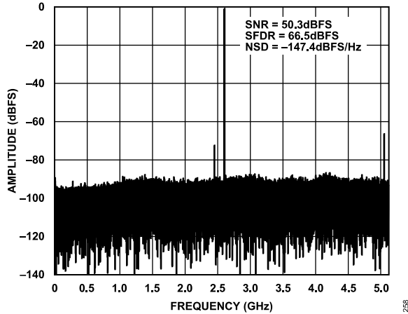
Figure 9. Single-Tone FFT with f_{IN} = 2.6 GHz, 10.25 GSPS
