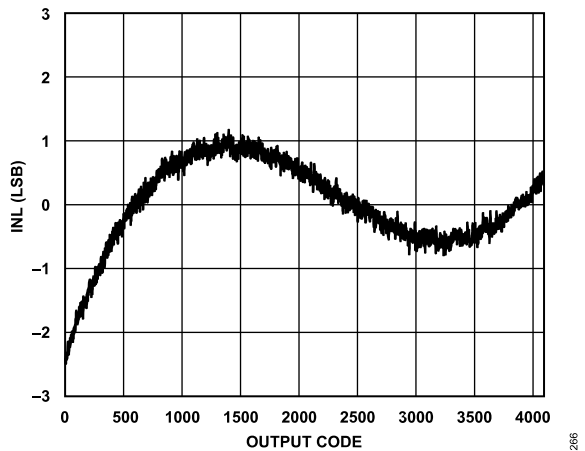
Figure 35. INL at f_{IN} = 170 MHz, 10 GSPS
