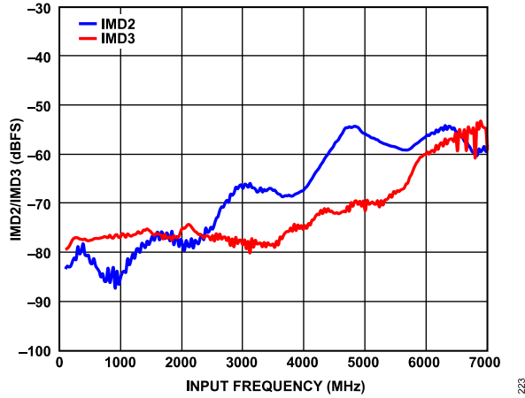
Figure 39. IMD2/IMD3 vs. Input Frequency ( A_{IN} = -7 dBFS), 10 MHz Spacing, 10 GSPS
