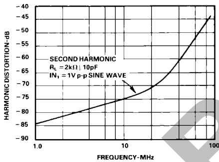
Figure 3. Harmonic Distortion vs. Frequency
