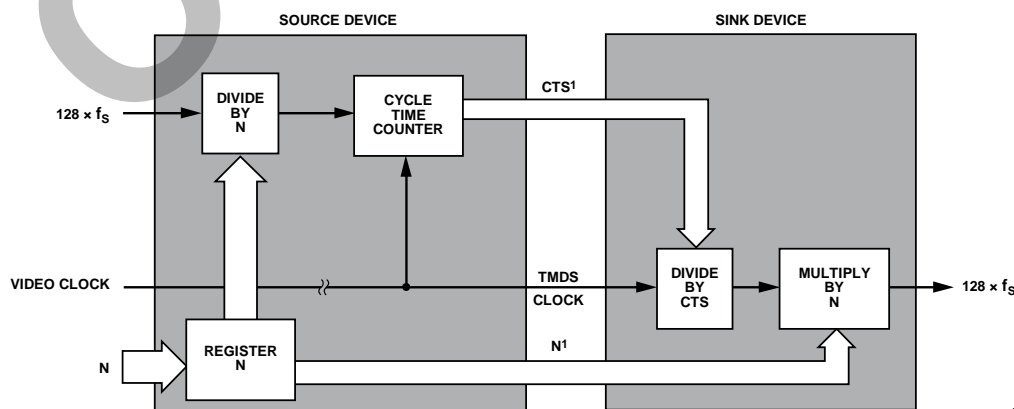
Figure 8. Audio Clock Regeneration
