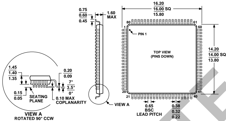
COMPLIANT TO JEDEC STANDARDS MS-026-BEC Figure 13. 80-Lead Low Profile Quad Flat Package [LQFP] (ST-80-2) Dimensions shown in millimeters
