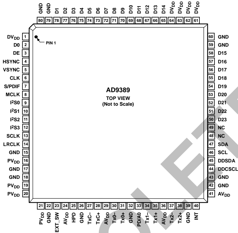
Figure 2. Pin Configuration
