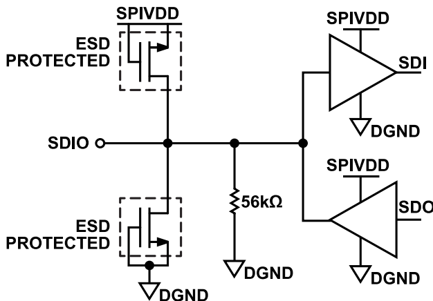
Figure 48. SDIO Input
