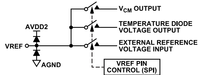
Figure 50. VREF Input/Output
