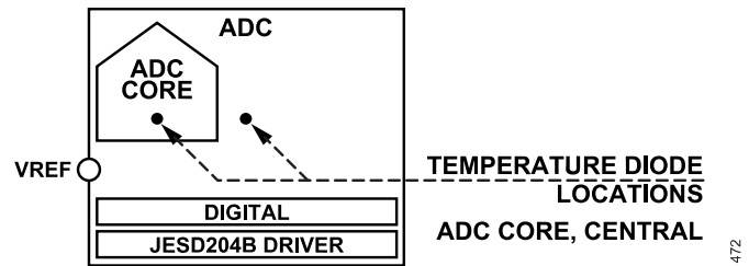
Figure 71. Temperature Diode Locations in the Die
