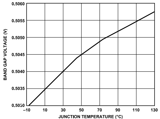
Figure 61. Typical V_{REF} Drift
