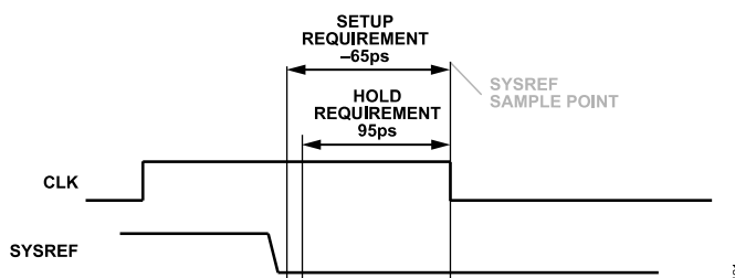
Figure 121. SYSREF High to Low Transition Using Falling Edge Clock Capture (Register 0x0120, Bit 4 = 1'b1, Register 0x0120, Bit 3 = 1'b0)
