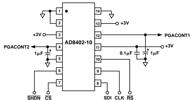
Figure 30. Digital Control of PGA
