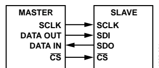
Figure 1. SPI Basic Interconnection
