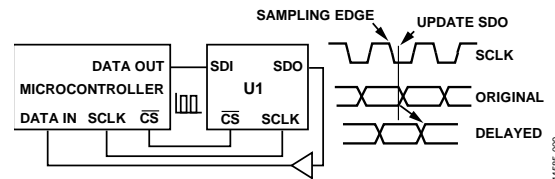
Figure 6. Enable Time
