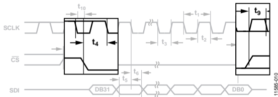
Figure 9. Enable and Disable Time
