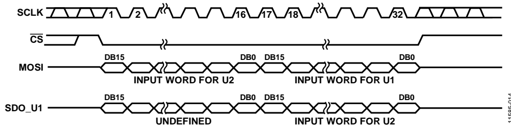
Figure 14. Daisy-Chain Timing Diagram
