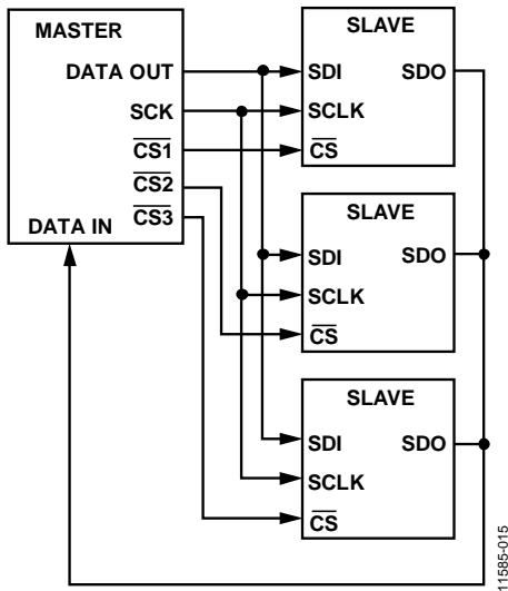
Figure 15. Parallel Configuration
