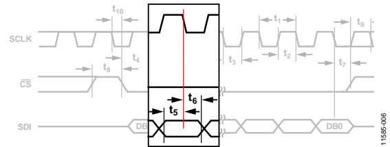
Figure 5. Phase Mode
