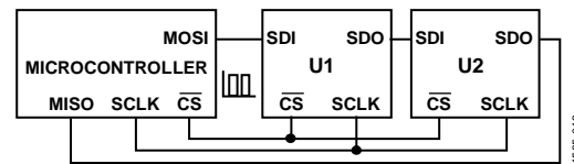
Figure 13. Daisy-Chain Configuration
