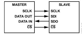
Figure 12. Standalone Configuration
