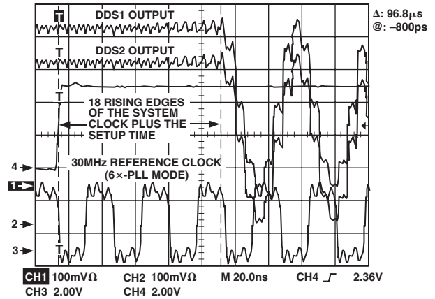
Figure 9. DDS Synchronization – Max System CLK (PLL Mode)
