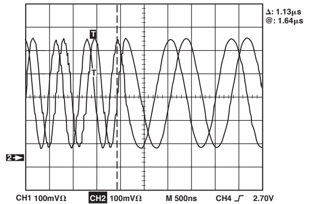
Figure 10. DDS Quadrature Synchronization
