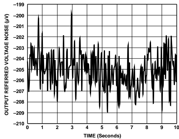
Figure 35. 1/f Noise for 0.1 Hz to 10 Hz Bandwidth, f_s = 100 \text{ kSPS} , 256 Samples Averaged per Reading, OSR = 4096
