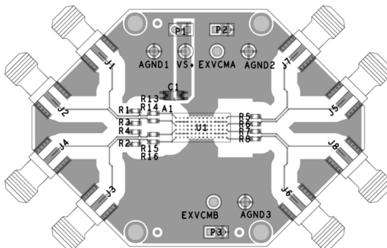
Figure 9. EVAL-ADAQ8088EBZ Top Copper Layer
