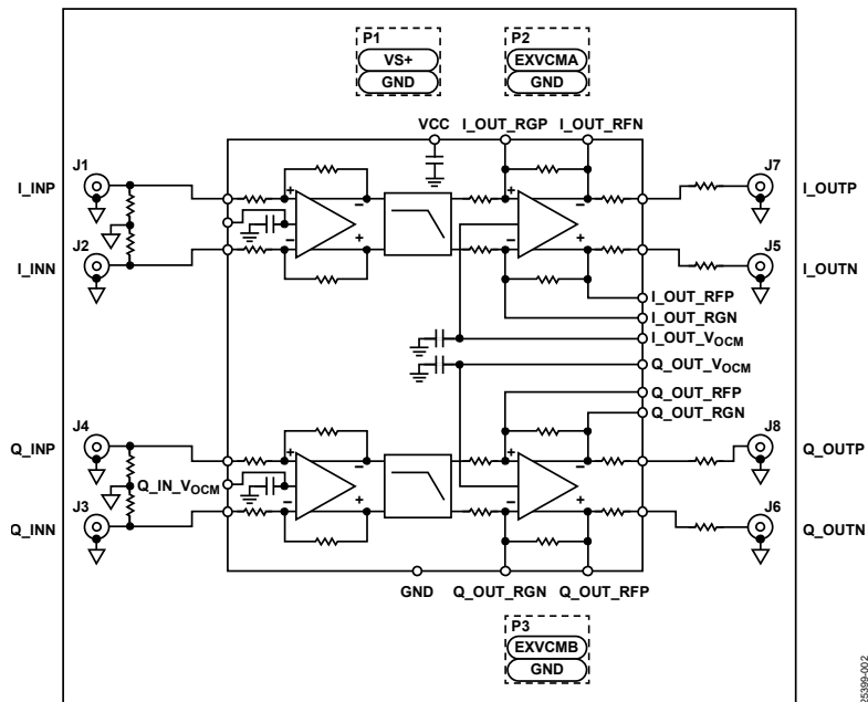
Figure 2. Simplified EVAL-ADAQ8088EBZ Block Diagram
