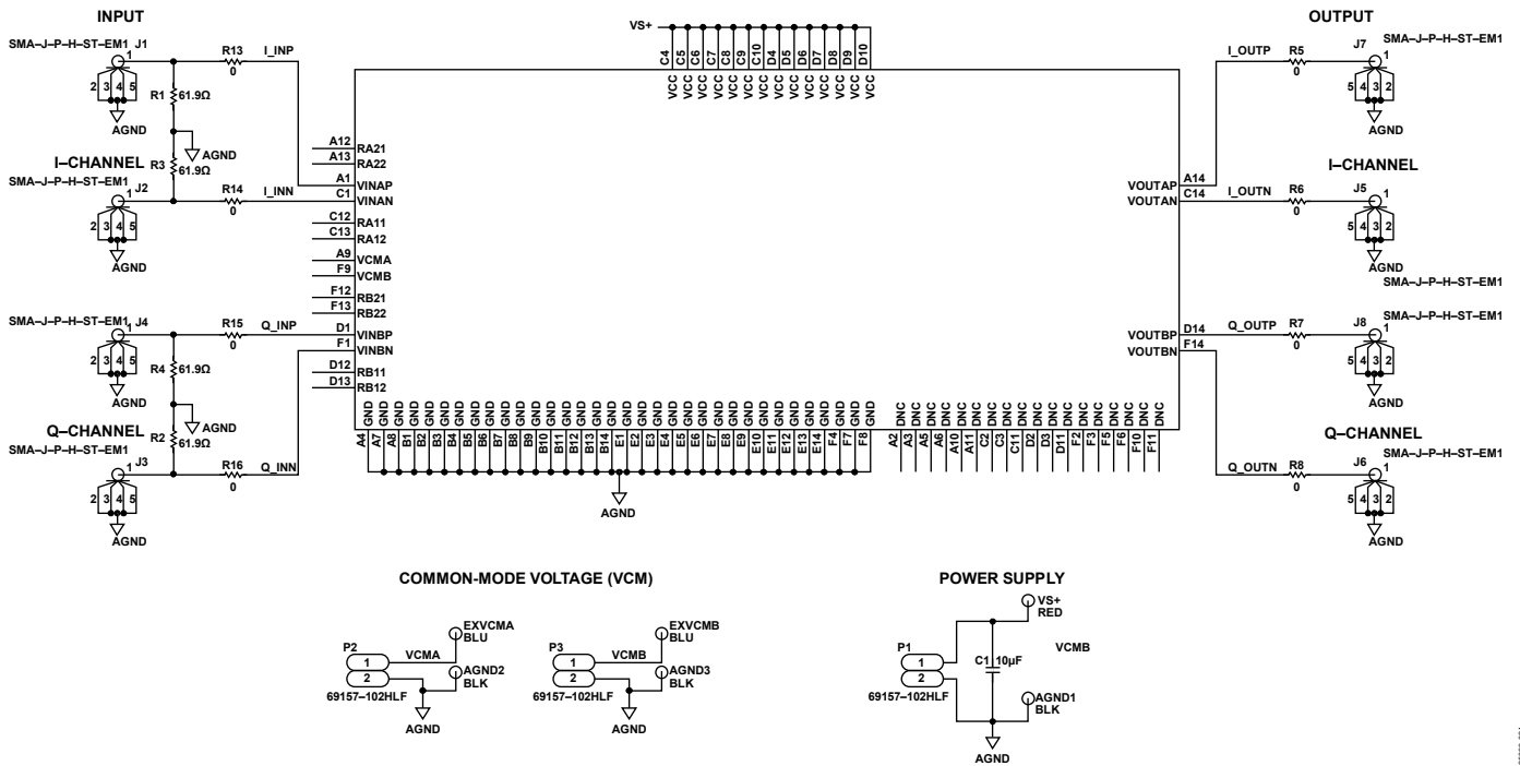
Figure 7. EVAL-ADAQ8088EBZ Schematic
