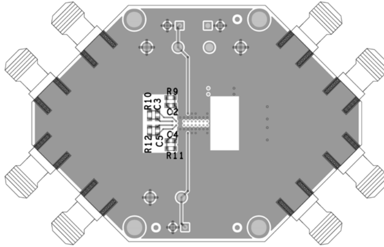
Figure 12. EVAL-ADAQ8088EBZ Bottom Copper Layer
