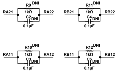
Figure 8. EVAL-ADAQ8088EBZ Feedback Resistor/Capacitor Placeholders
