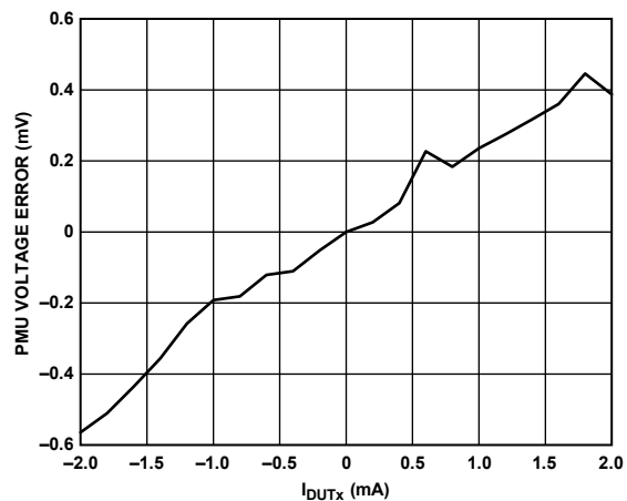
Figure 50. PMU FV Range B Output Voltage Error at 6.75 V vs. Output Current
