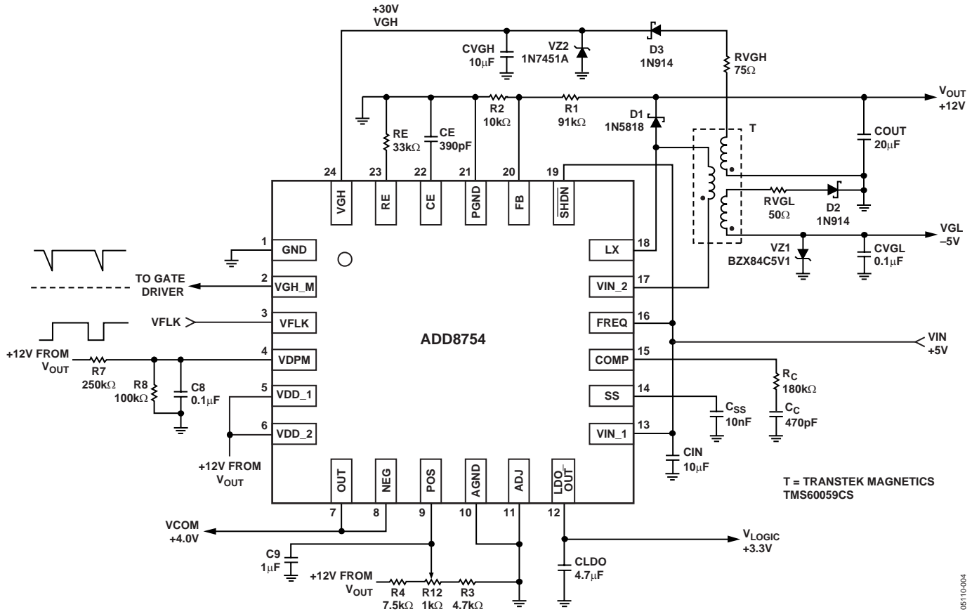
Figure 24. 1.2 MHz Application Circuit for TFT LCD Display with Transformer for VG and VGL
