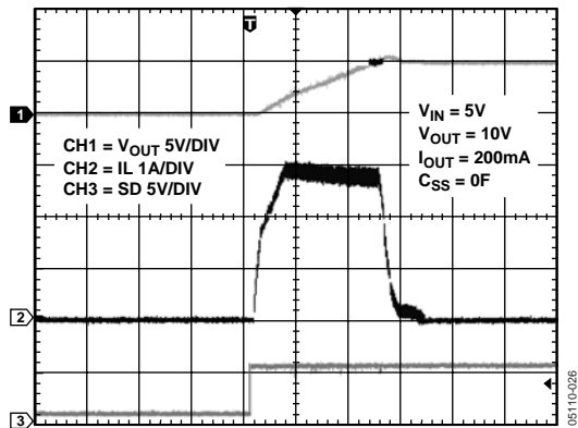
Figure 4. Start-Up Response from Shutdown, C_{SS} = 0F
