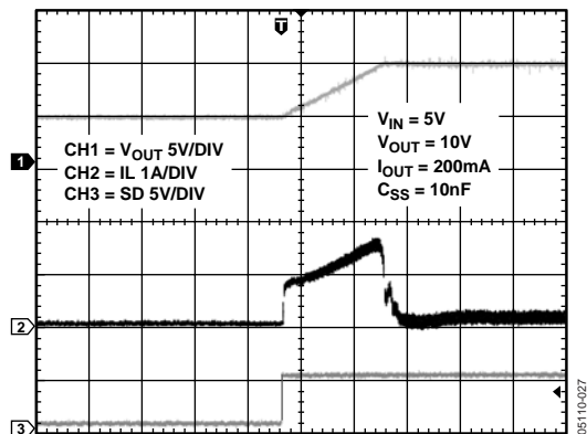
Figure 5. Start-Up Response from Shutdown, C_{SS} = 10F
