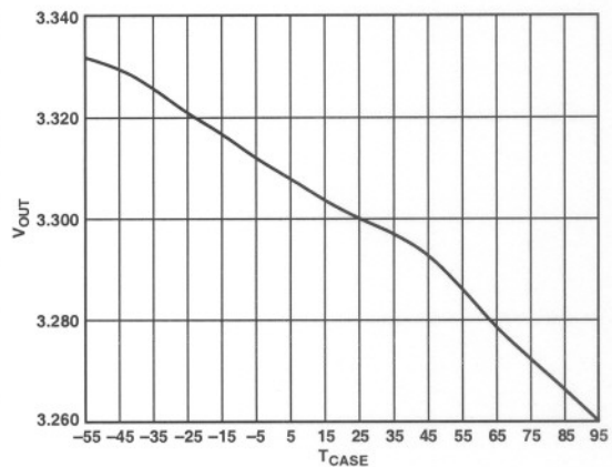
Figure 6. Output Voltage vs. Case Temperature (°C) (ADDC02803SC)
