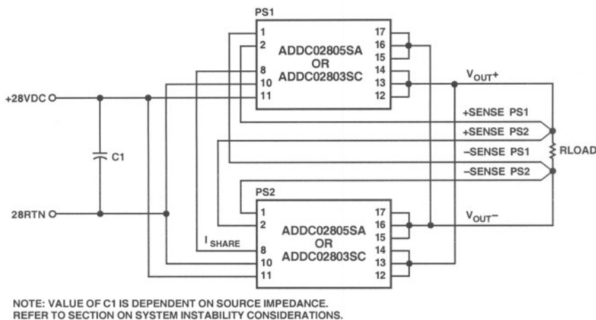
Figure 37. Typical Connections for Paralleling Two Converters
