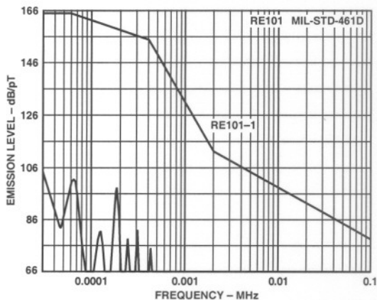
Figure 21. Radiated Emissions, MIL-STD-461D, RE101, 100 W Load
