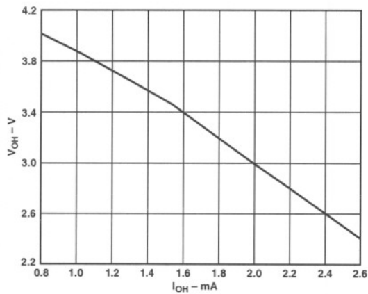
Figure 27. Source Capability of Status Output (ADDC02805SA)
