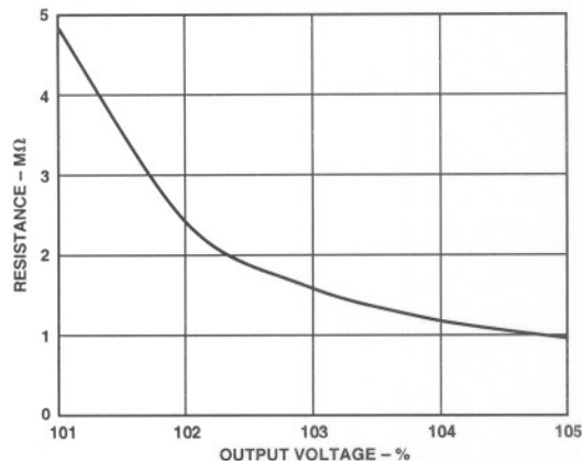
Figure 25. External Resistor for Increasing Output Voltage
