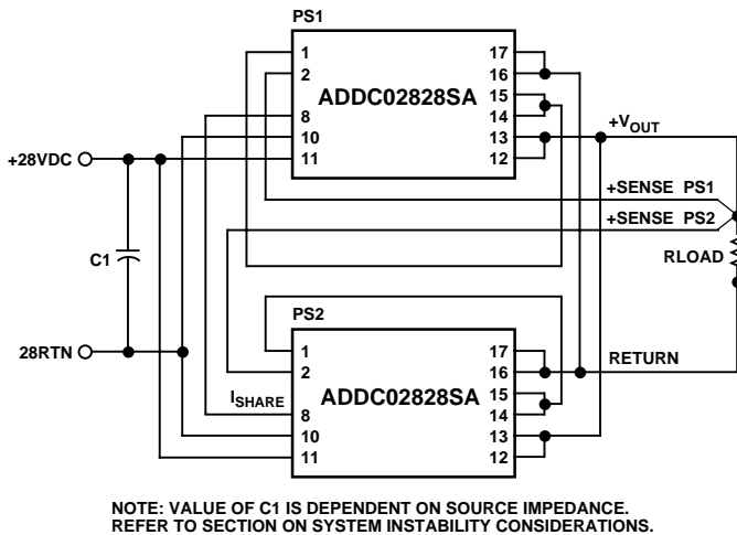
Figure 27. Typical Connections for Paralleling Two Converters (+28 V dc Out)
