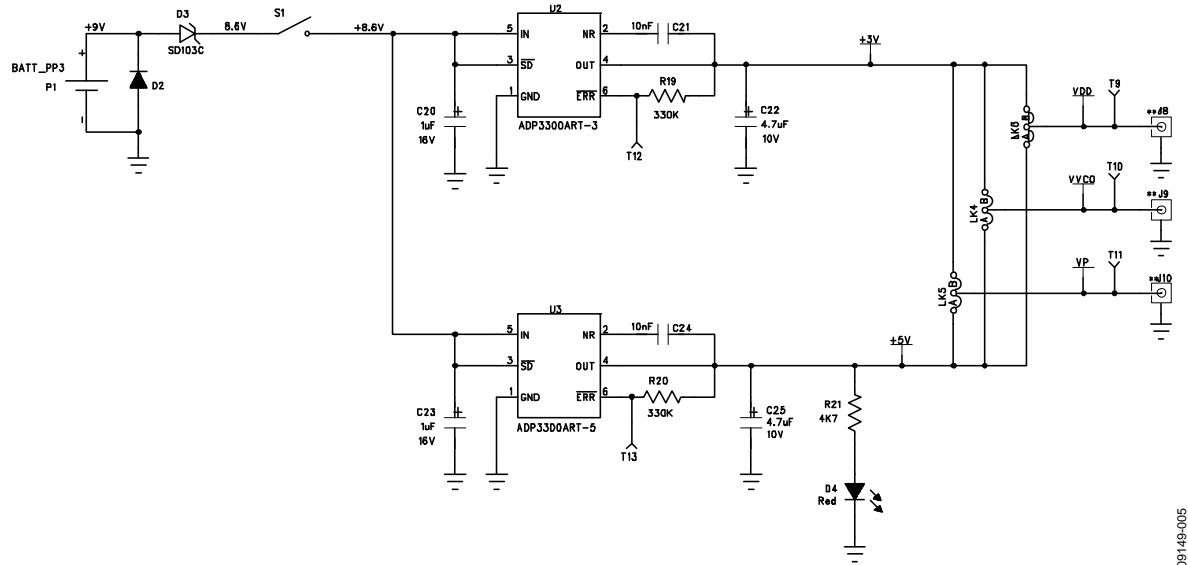
Figure 6. Evaluation Board Circuit Diagram (Part 2)
