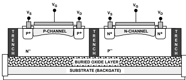
Figure 12. Trench Isolation
