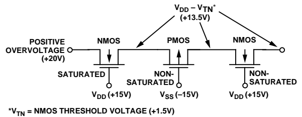
Figure 8. Positive Overvoltage on the Channel Protector
