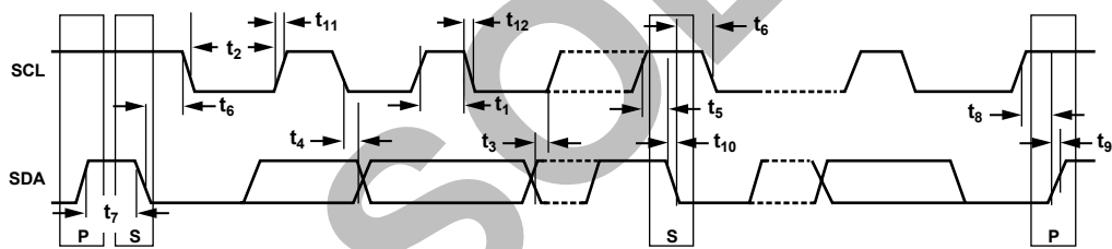
Figure 2. Timing Diagram for 2-Wire Serial Interface
