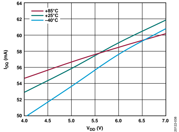
Figure 38. I_{DQ} vs. V_{DD} for Various Temperatures
