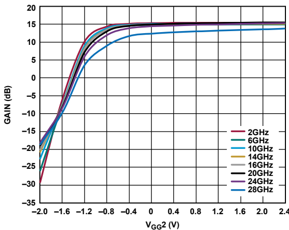
Figure 10. Gain vs. V GG2 for Various Frequencies
