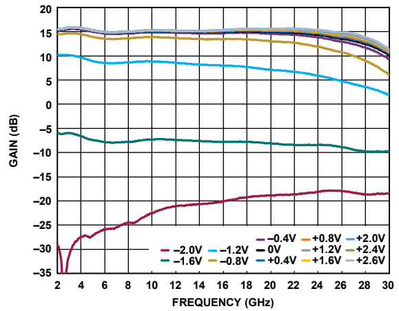
Figure 12. Gain vs. Frequency at Various V GG2 Voltages
