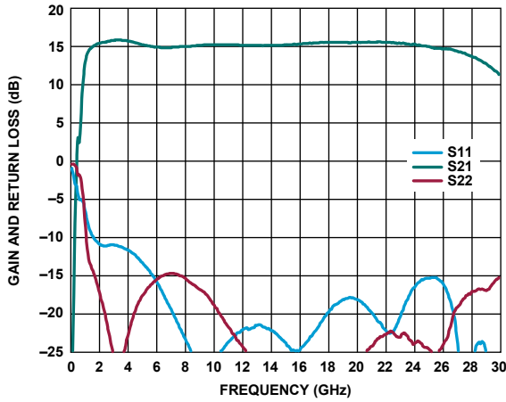
Figure 8. Gain and Return Loss vs. Frequency
