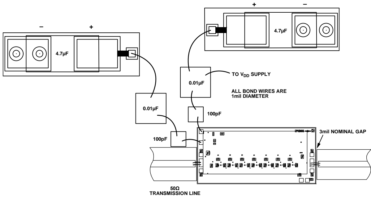
Figure 42. Assembly Diagram
