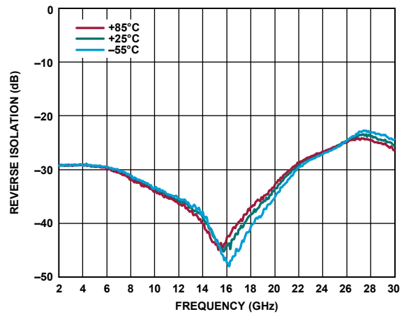
Figure 13. Reverse Isolation vs. Frequency at Various Temperatures
