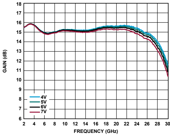
Figure 9. Gain vs. Frequency at Various Supply Voltages
